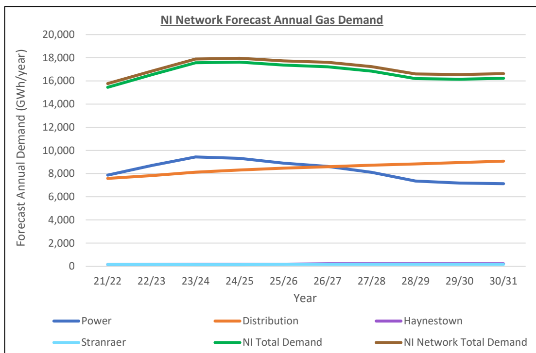
Figure 4-9: NI Network Forecast Annual Demand for Gas Years 2020/21 to 2030/31 (GWh/day)
