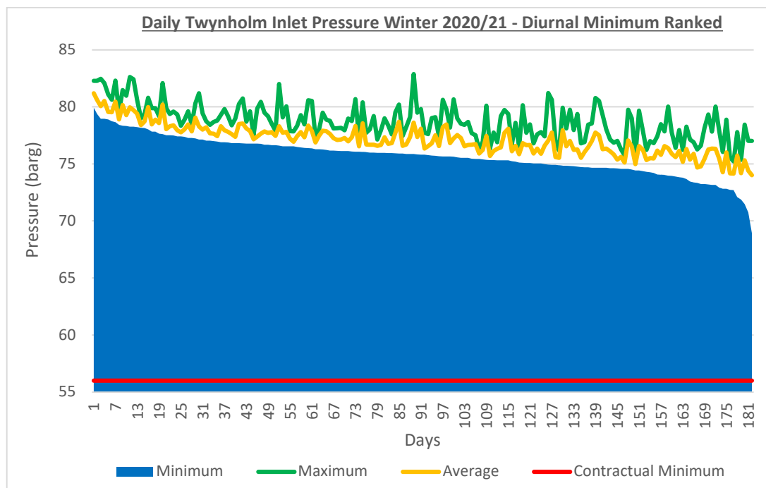
Figure 5-2: Duration Curve of Twynholm Inlet Pressure Winter 2020/21
